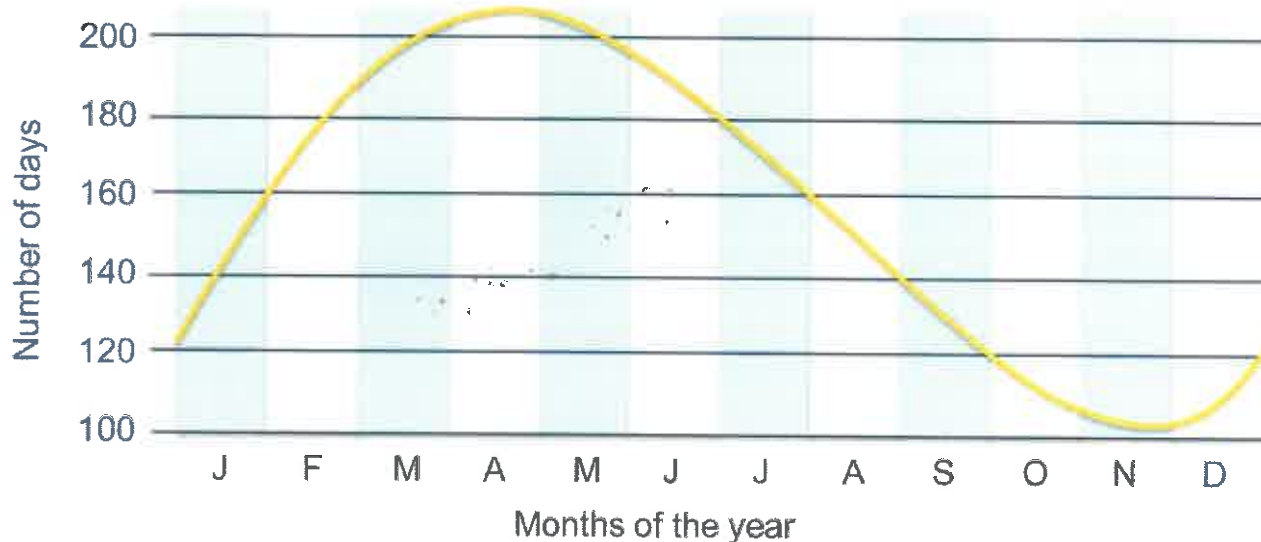
Figure 2. Approximate number of days from flowering to harvest for subtropical bananas over a 12-month period. Time period is for bunches emerging during the indicated month. Drawn from Robinson and Galán Saúco (2010).
