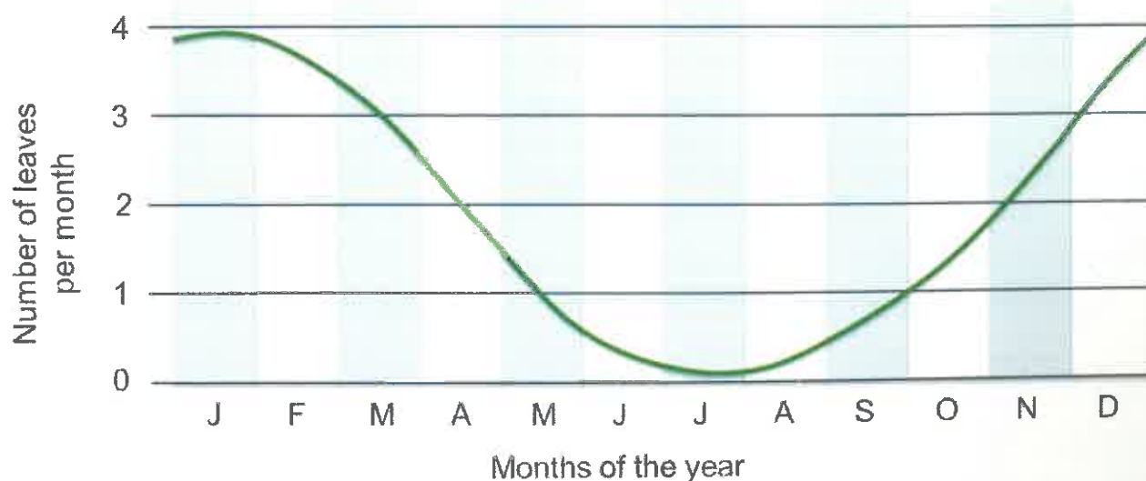
Figure 1. Monthly leaf emergence rate for subtropical bananas over a 12-month period. Drawn from Robinson and Galán Saúco (2010).
