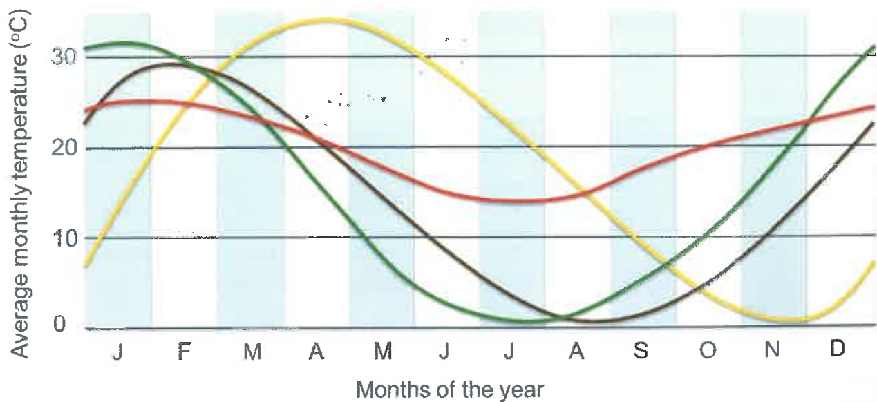
Figure 4. Combined phenological events for subtropical bananas over a 12-month period plotted against average monthly temperature for Coffs Harbour. Axis scales for the growth curves are as for figures 1 to 3. Drawn from Robinson and Galán Saúco (2010).
